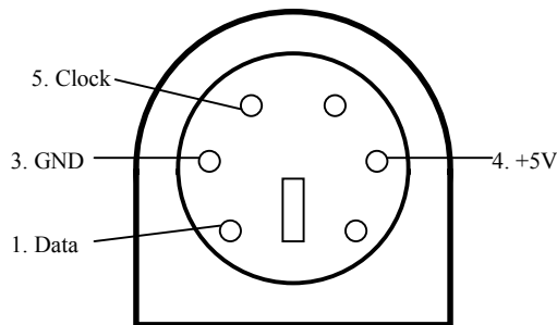
6-Pin mini-DIN male connector. Viewed looking into connector.
