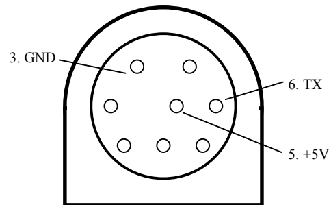
6-Pin mini-DIN male connector. Viewed looking into connector.
